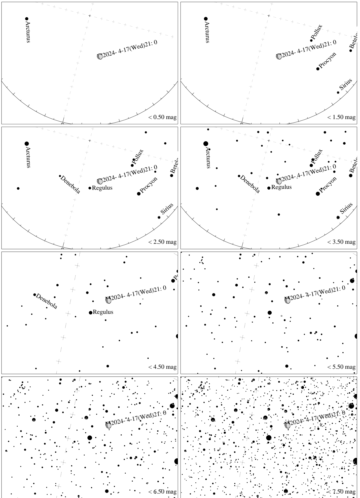
Maps for Globe at Night at latitude 50^\circ , 2024-04-17, 21 h local time (Sun at -18^\circ ), transparent air. Lines from N(E,S,W) to zenith shown (crosses each 10^\circ ). Regulus ( \alpha Leonis) is 14^\circ to the right from S, at 51^\circ height. Detailed maps 50^\circ vertically, the first four maps 100^\circ . Jan Hollan maps, CzechGlobe
